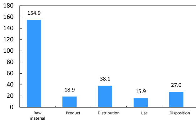
Warming load CO 2 equivalent of each stage[kg]
