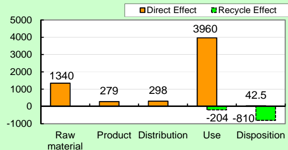
Warming load CO 2 equivalent of each stage [ kg ]
